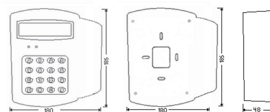
Dimension (mm)
